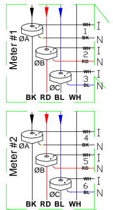
Diagram 1. Current Transformers installed inside tenant breaker panel.
