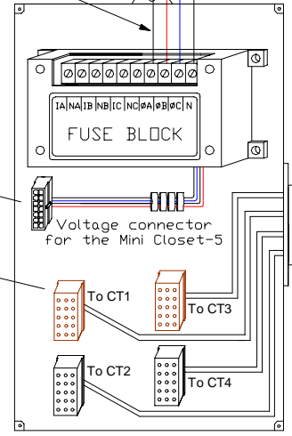
Diagram 1. Current Transformers installed inside tenant breaker panel.
