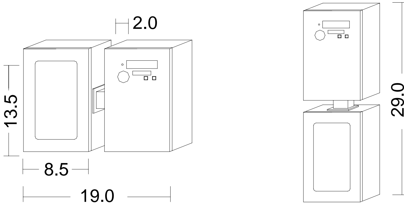
MiniCloset-5 Dimensions (Choose the orientation best suited for the installation site.)
